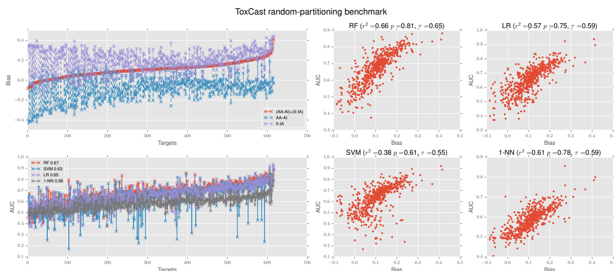
Figure 10: Illustration of the performance of four commonly used classification algorithms: Random-Forests (RF), Logistic Regression (LR), Support Vector Machines (SVM), and K-Nearest-Neighbors (KNN) over the ToxCast benchmark 34 using random partition cross-validation. Each ML algorithm shows clear correlation between AVE bias and AUC (see text for discussion). Top left: calculated AVE bias for phenotypic conditions. Bottom left: AUC performance of the different algorithms over the 617 phenotypes ordered by their corresponding AVE bias values. Right: scatter plots of the correlation between AUC and AVE bias for each of the classification algorithm over the 617 targets.
