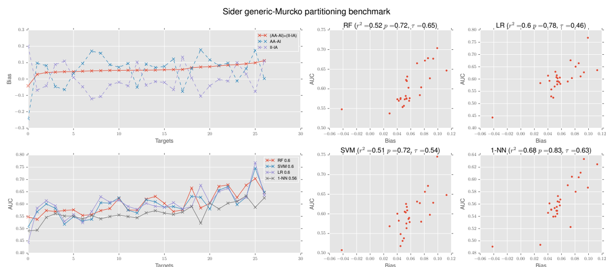
Figure 13: Illustration of the performance of four commonly used classification algorithms: Random-Forests (RF), Logistic Regression (LR), Support Vector Machines (SVM), and K-Nearest-Neighbors (KNN) over the Sider benchmark 34,36 using generic-Murcko partition cross-validation. Each ML algorithm shows clear correlation between AVE bias and AUC (see text for discussion). Top left: calculated AVE bias for 27 benchmark targets. Bottom left: AUC performance of the different algorithms over the 27 ADR classes ordered by their corresponding AVE bias values. Right: scatter plots of the correlation between AUC and AVE bias for each of the classification algorithm over the 27 targets.
